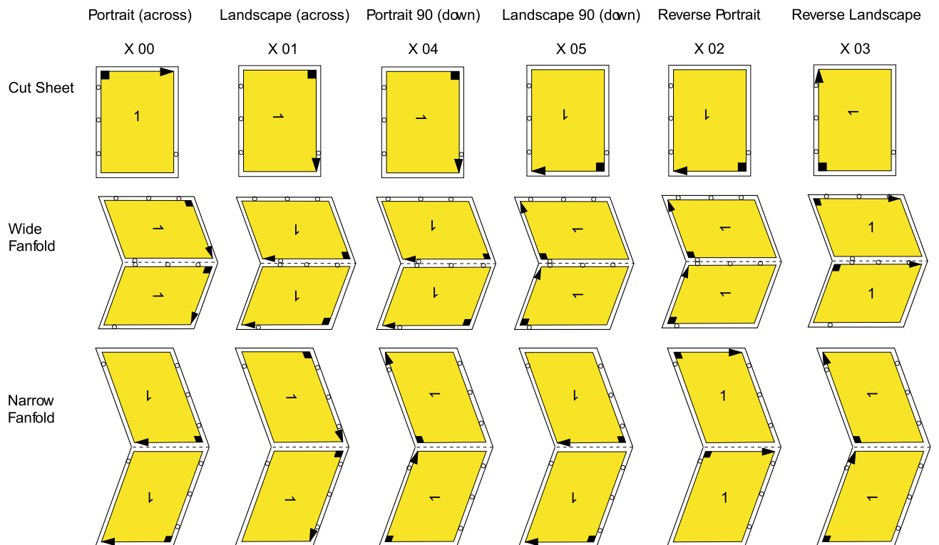
Figure 69. 1-up Partition Numbering, Back Sheet-Side, Tumble Duplex
