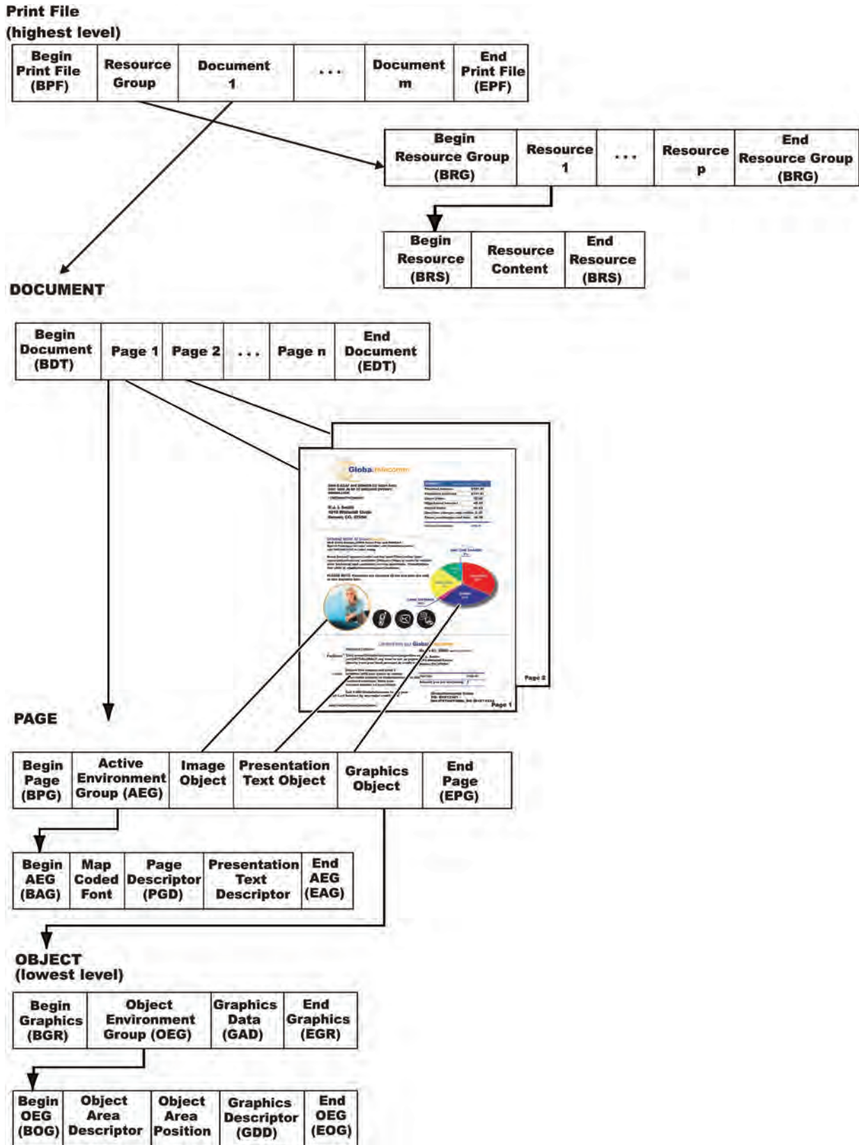
Figure 4. MO:DCA Presentation Document Components
