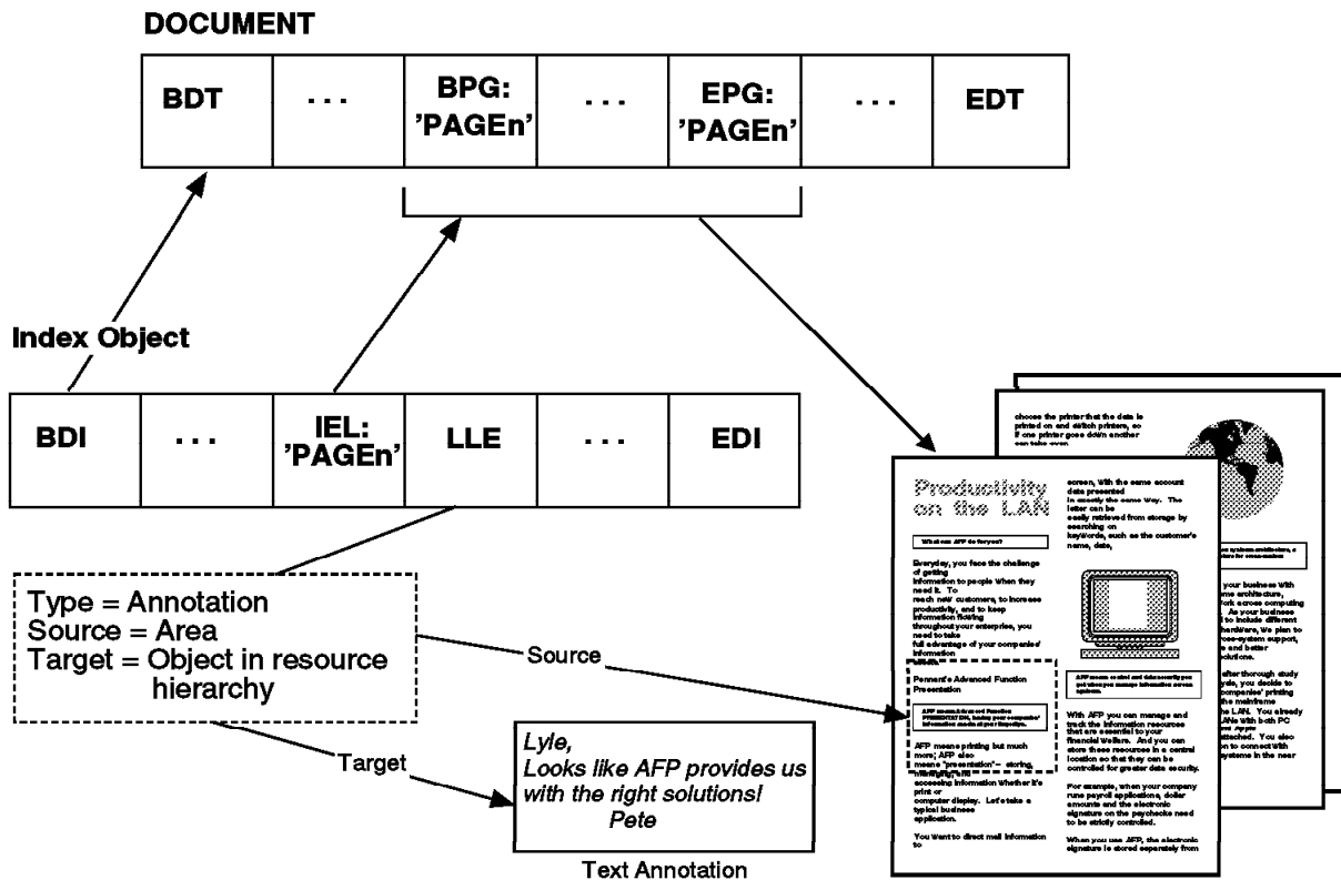
Figure 20. Document Annotation using the LLE
