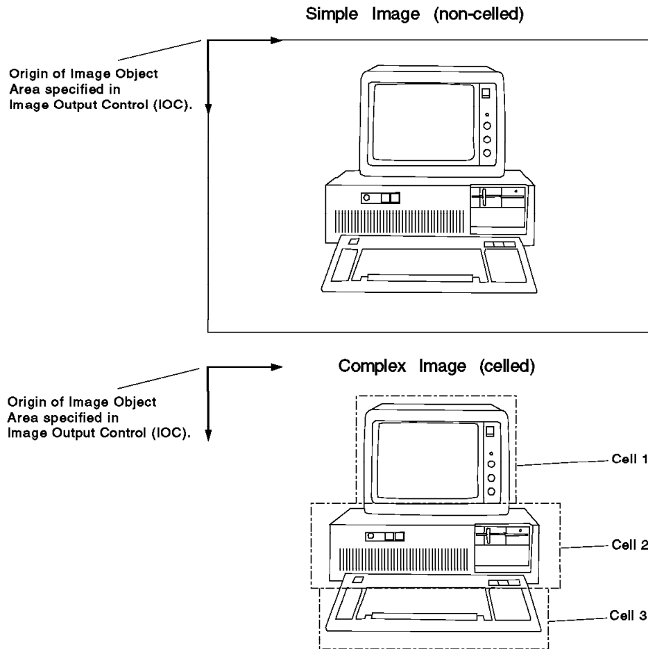
Figure 103. Two Forms of IM Image
