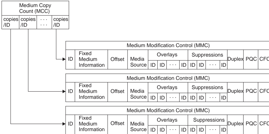
Figure 35. Copy Subgroups
